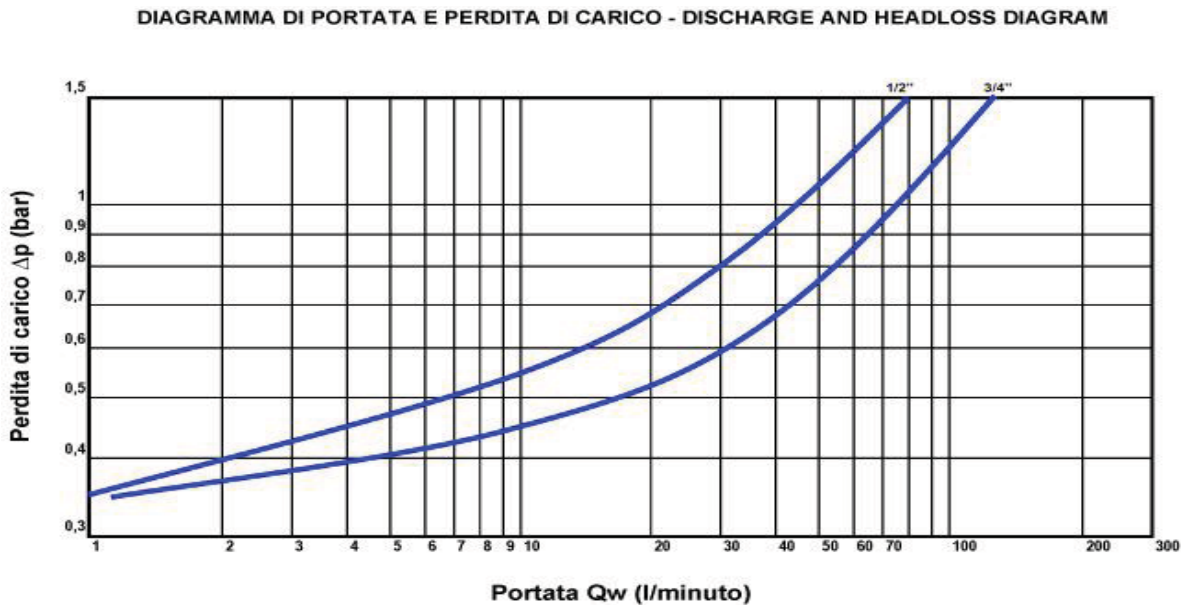
Flow Rate vs Pressure Drop Chart
