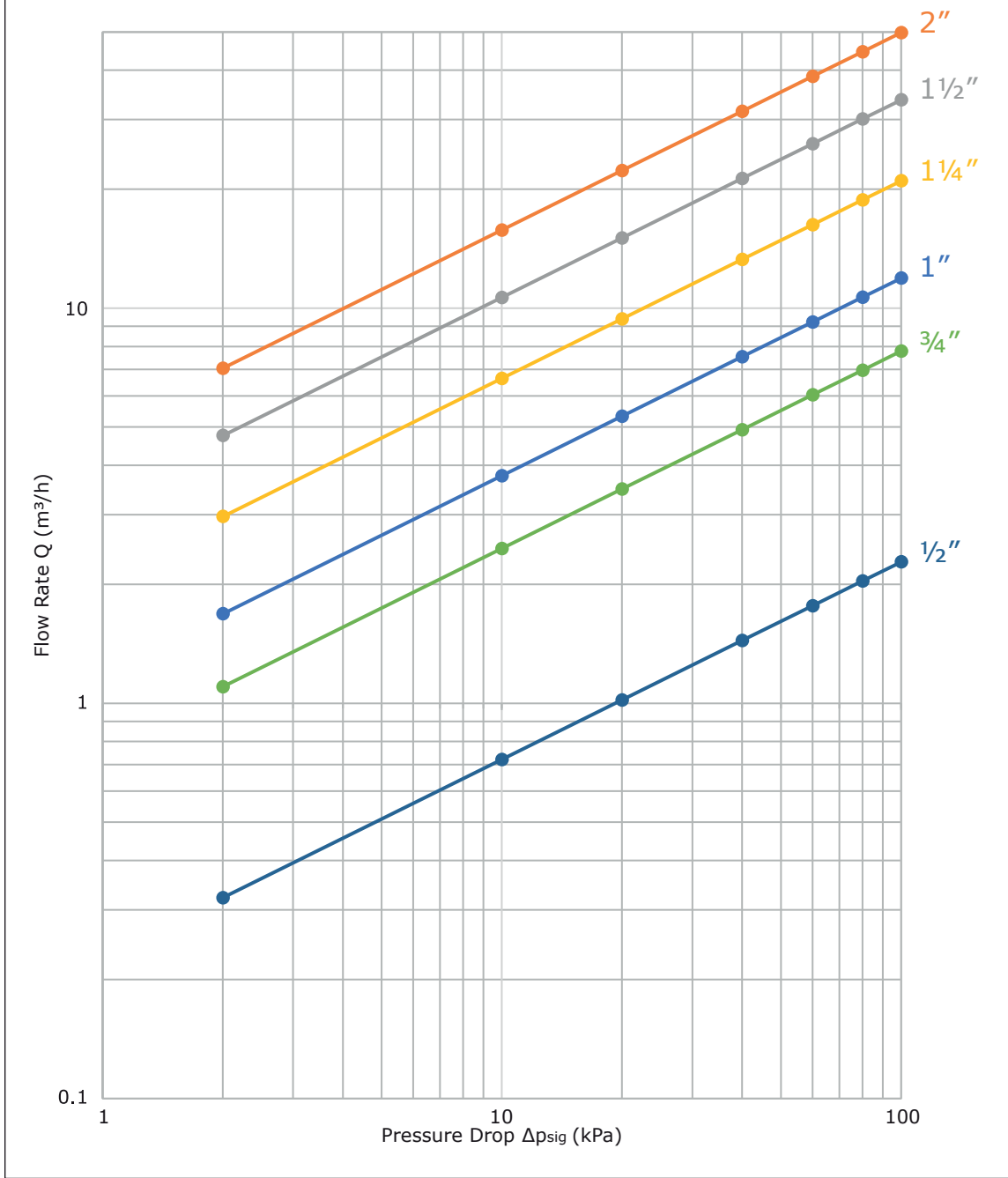
Kvsig Chart
